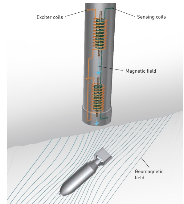
Passive magnetometer methods
