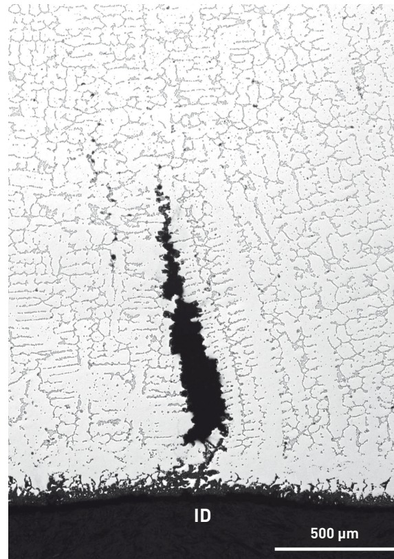
Figure 7: Higher magnification photomicrograph of creep fissure
