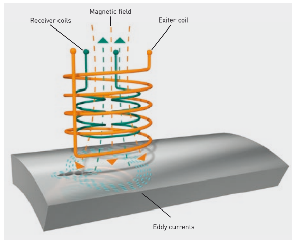
Figure 6: The principle behind eddy current testing
